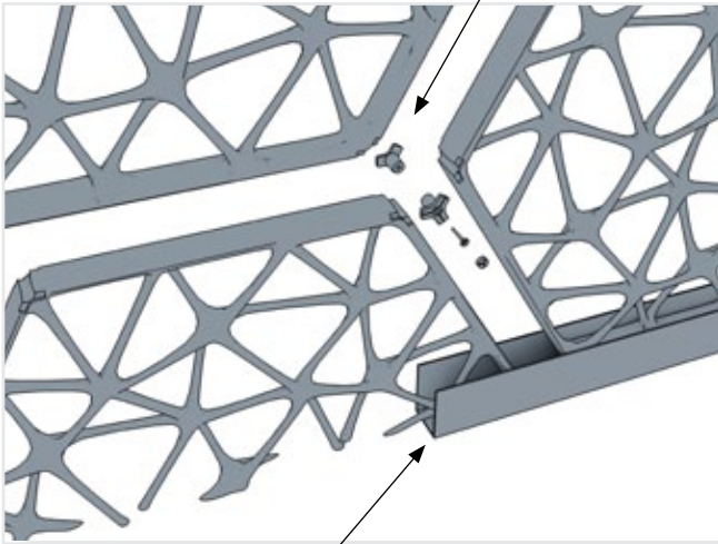
Connection system
